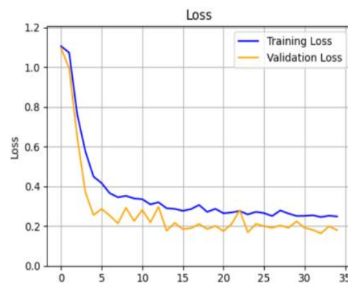
Figure 5. Proposed Model Loss
